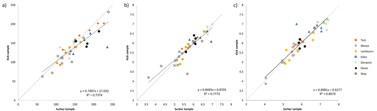
Fig. 4. Relationships between the (a) BMWP, (b) ASPT and (c) WHPT calculated using data from Surber versus kick samples, taken on the same day and at the same site. Points are colour-coded to designate the river where the sample was taken.
