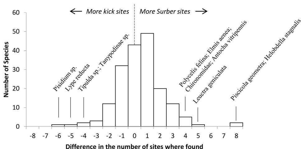
Fig. 7. The difference in the number of sites where taxa were caught between kick and Surber samples. Taxa that were found at four or more additional sites for one method are labelled. Zero indicates the taxa was found in the same number of kick and Surber samples.
