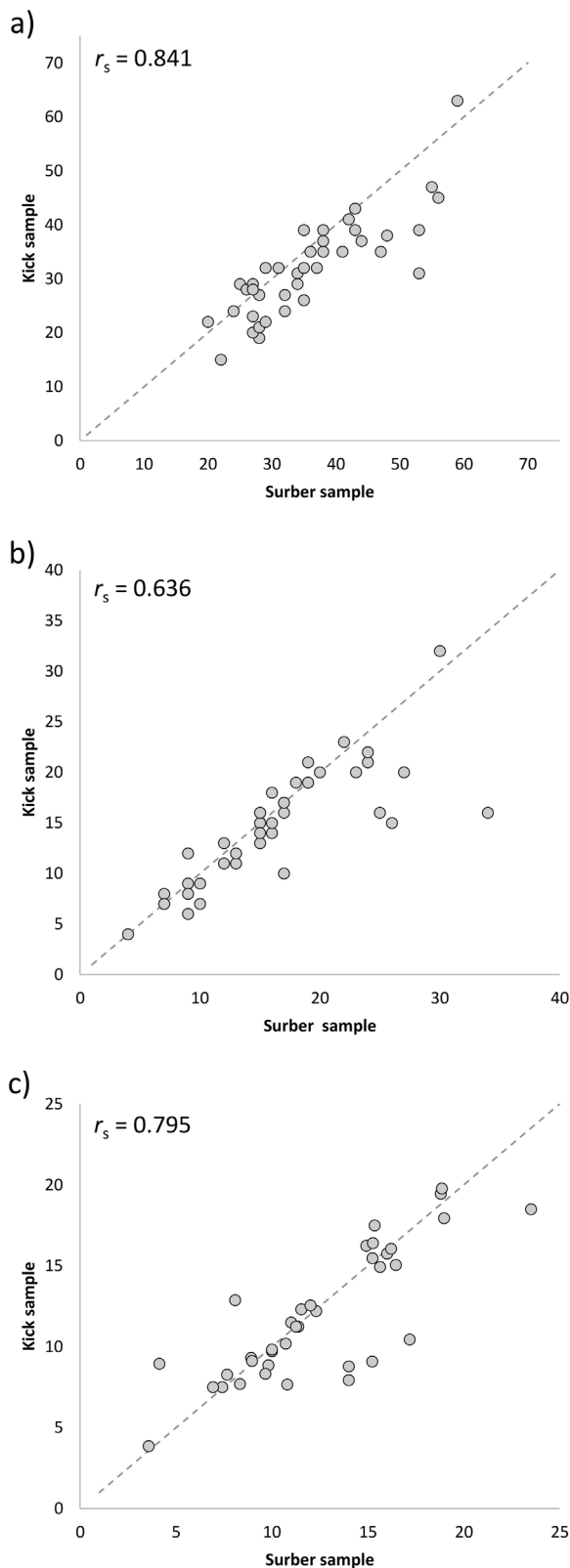
Fig. 3. Relationship between a) taxa richness, b) EPT richness (e.g. mayfly, stonefly and caddisfly; EPT) and c) the CCI collected in Surber and kick samples, taken on the same day and at the same site. Spearman ( r_s ) correlation coefficients are included.
