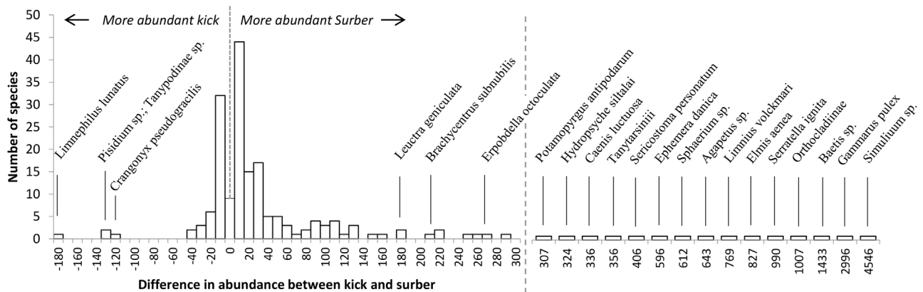
Fig. 6. The difference in abundance between kick and Surber samples for invertebrate taxa, aggregated across all sites. Note that the right-hand grey dashed line marks a transition in the horizontal axis from categorical values to absolute values. Taxa of note due to large differences between kick and Surber samples are labelled. Note that in some cases taxa were grouped to genus level (e.g. Baetis sp.) because differences in the proportion of individuals successfully identified to species level (as opposed to genus level) could otherwise have biased results.
