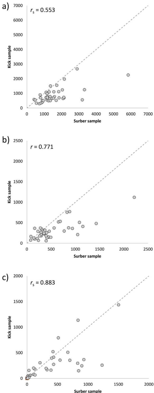
Fig. 2. Relationship between the a) total invertebrate abundance, b) total EPT and c) total Gammarus collected in Surber samples versus kick samples, taken on the same day and at the same site. Pearson ( r ) and Spearman ( r_s ) correlation coefficients are included for normal and non-parametric data, respectively.
