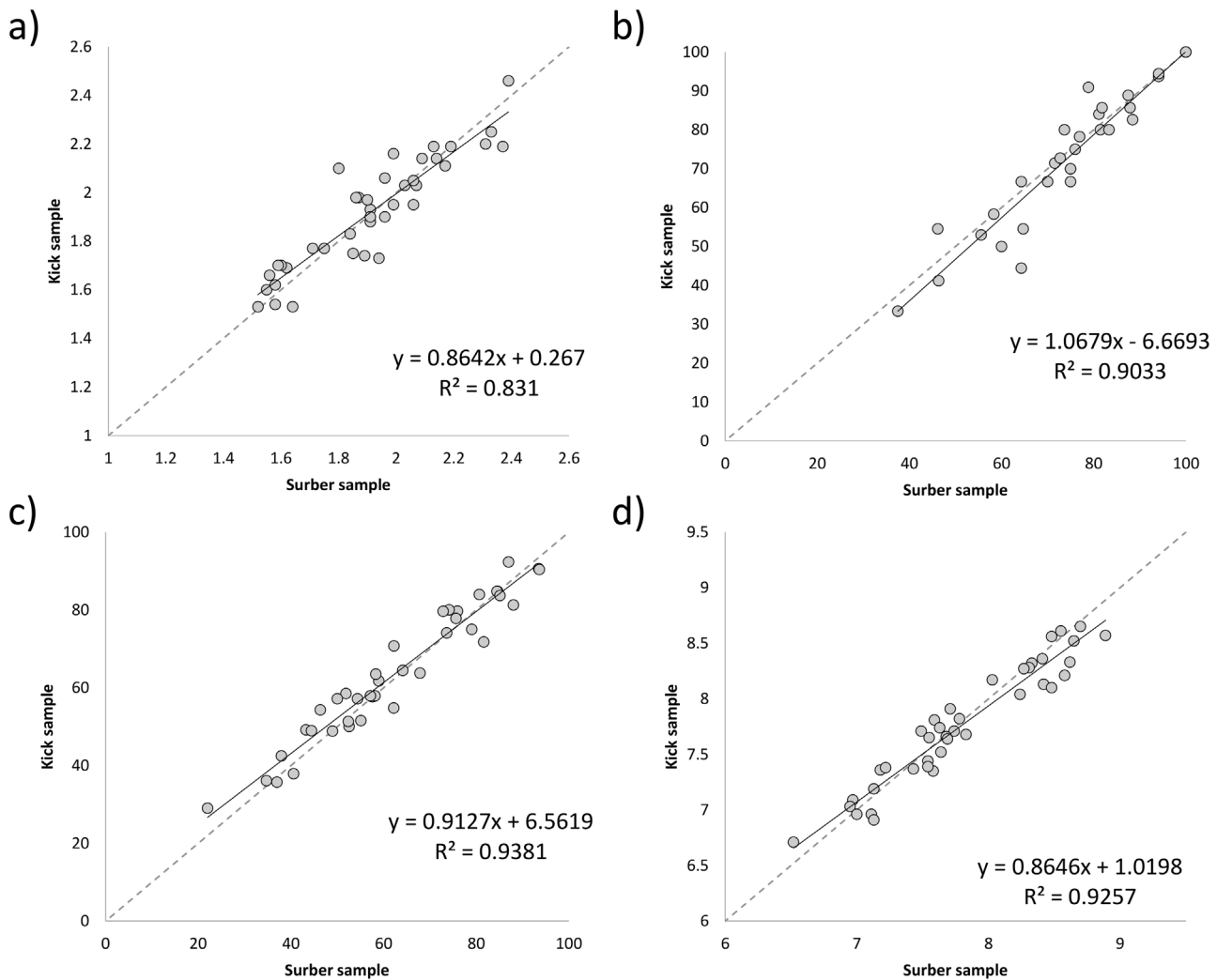
Fig. 5. Relationships between a) the Saprobic index, b) the TRPI, c) PSI and d) LIFE score calculated on Surber and kick samples, taken on the same day and at the same site.
